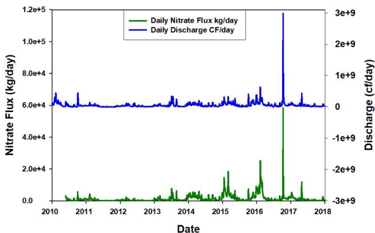
Figure 6. Nutrient flux at the Tomahawk River in the Cape Fear Basin.
